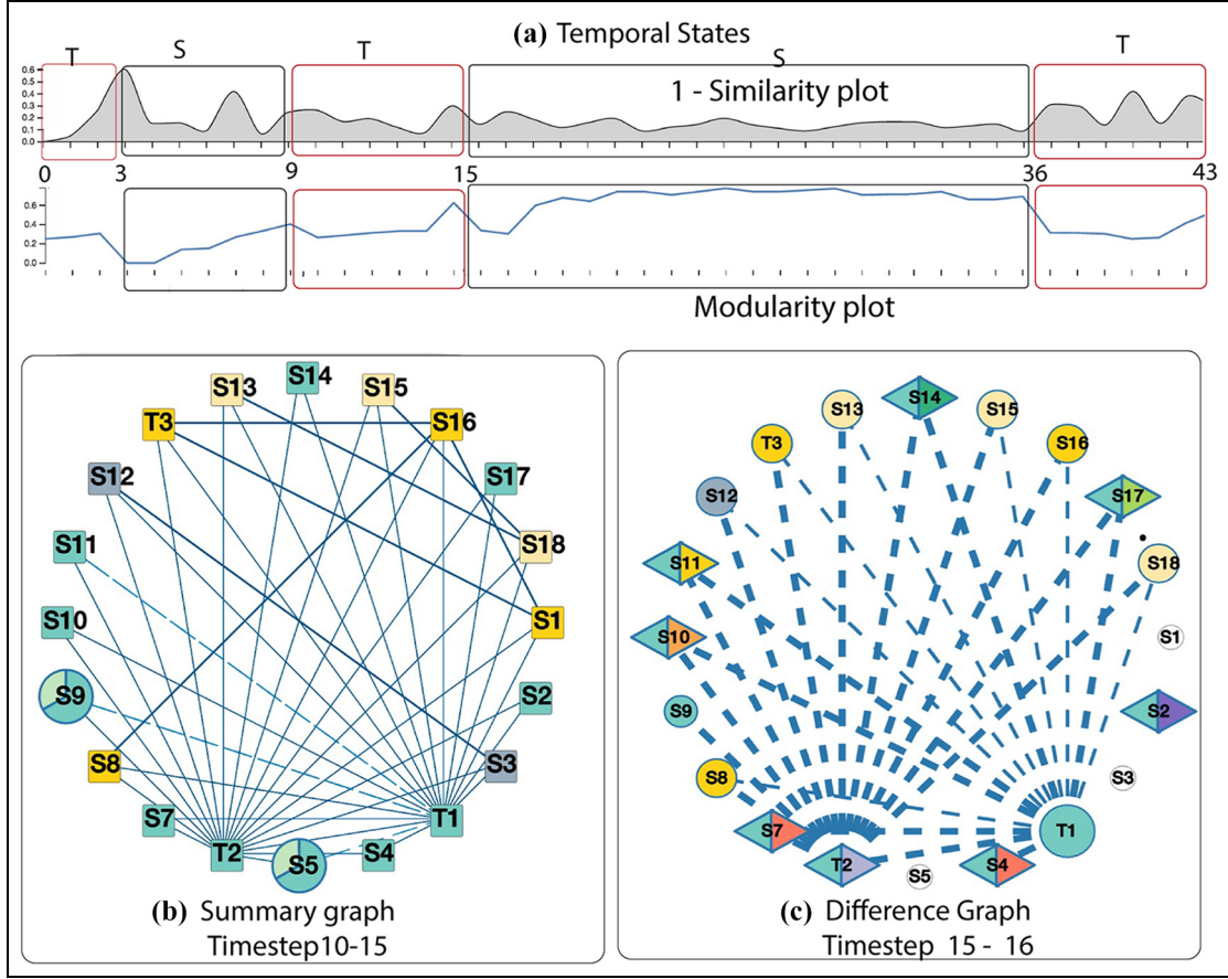
Figure 5. The two dominant states in the McFarland data set. (a) Red rectangles represent lecture sessions by the teachers, and black rectangles represent states when the teachers are not lecturing. (b) Broadcasting edges from teachers T1 and T2 depict lecturing student groups. (c) State change as a consequence of students forming groups and teachers not lecturing.
