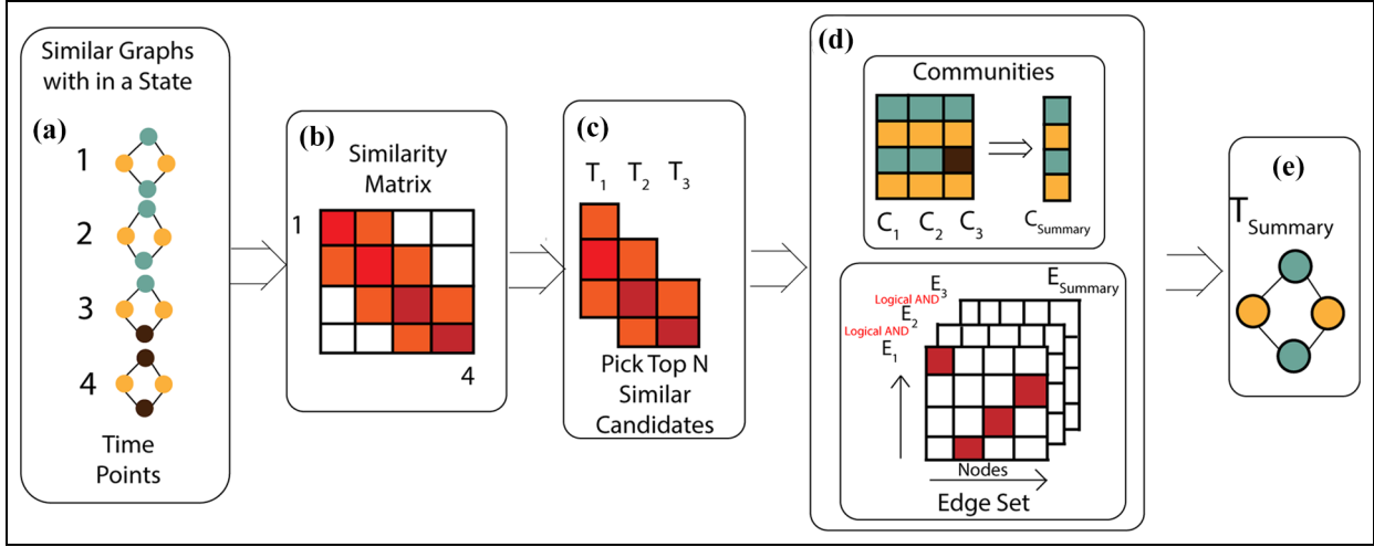
Figure 2. The algorithm used to construct the summary graph identifies the most common local and global topological attributes from a set of similar graphs.
